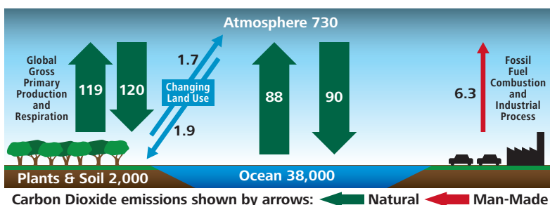
Figure 2. Global Carbon Flows and Sinks in billions of metric tons.
