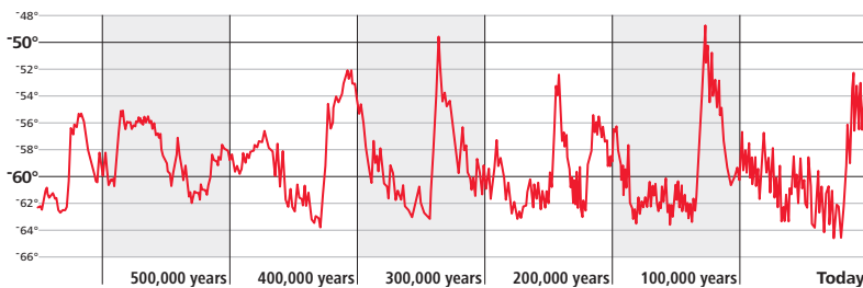
Figure 1. Antarctic ice core sample temperatures in Celsius.
